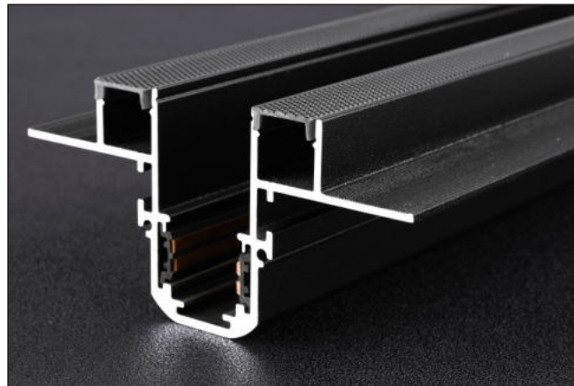
multi track embedded
