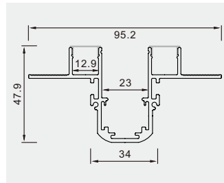
combined track embedded
